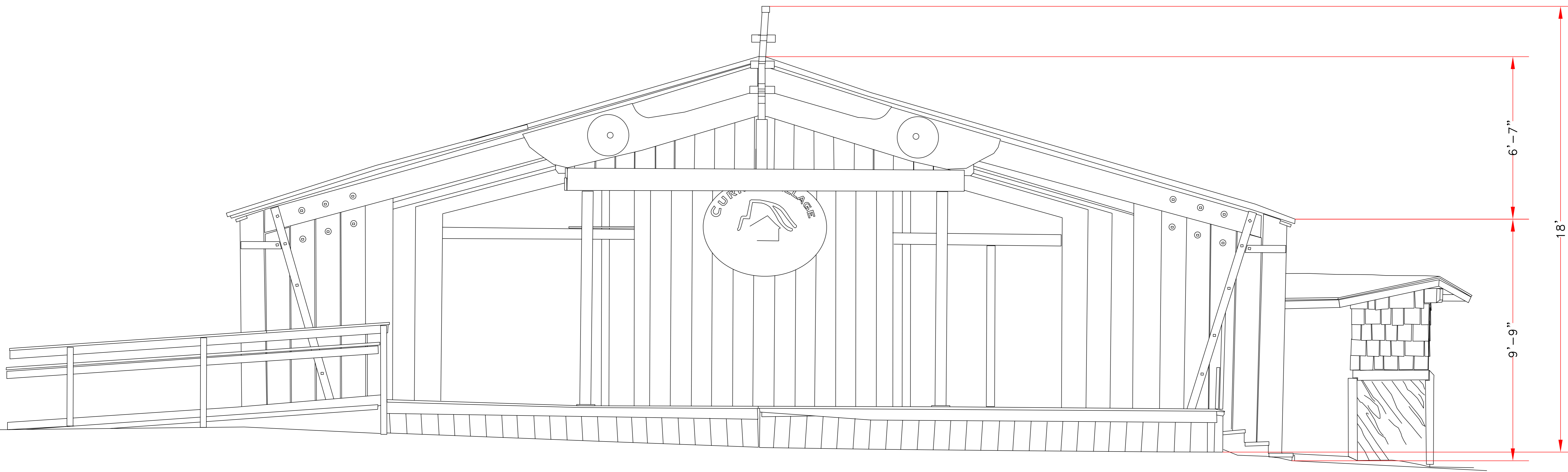
AMPHITHEATER – SOUTH ELEVATION
