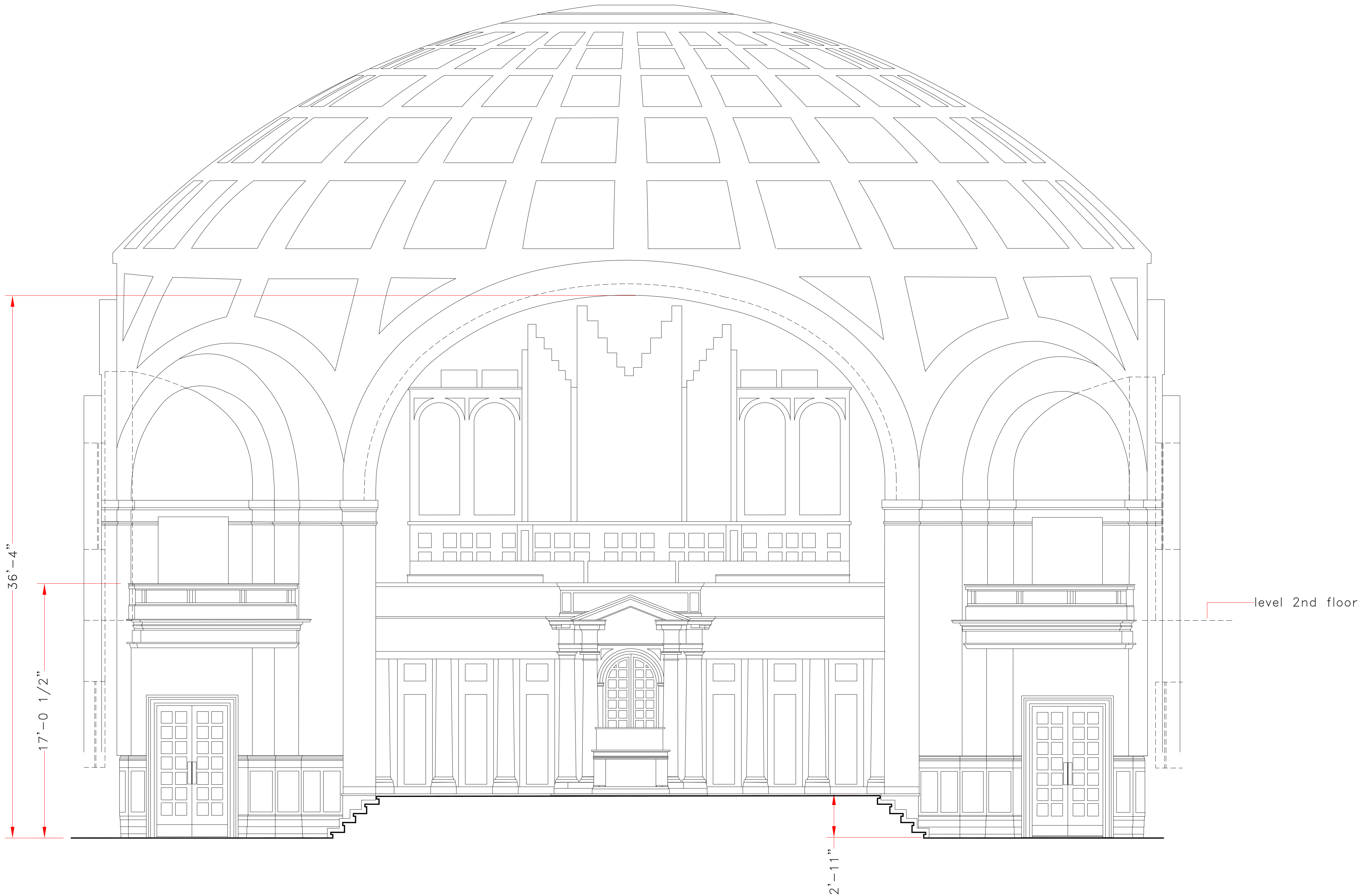
North elevation
