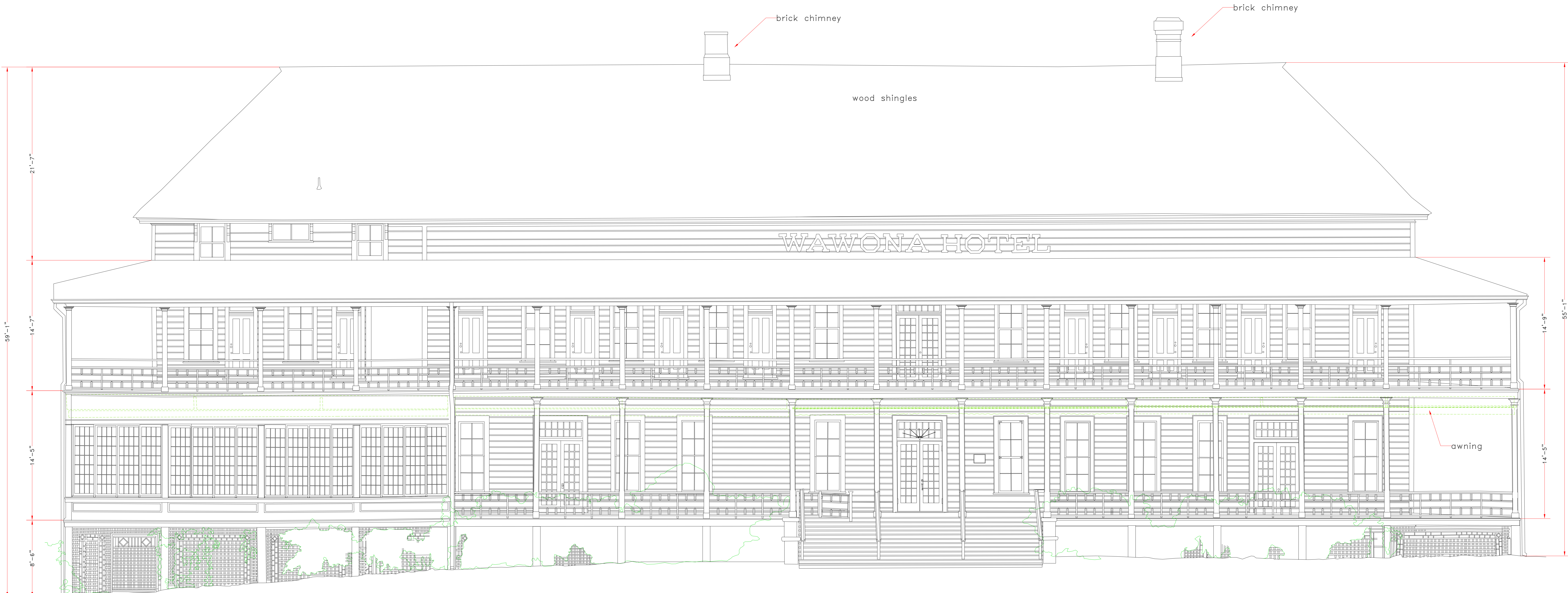
WEST ELEVATION
