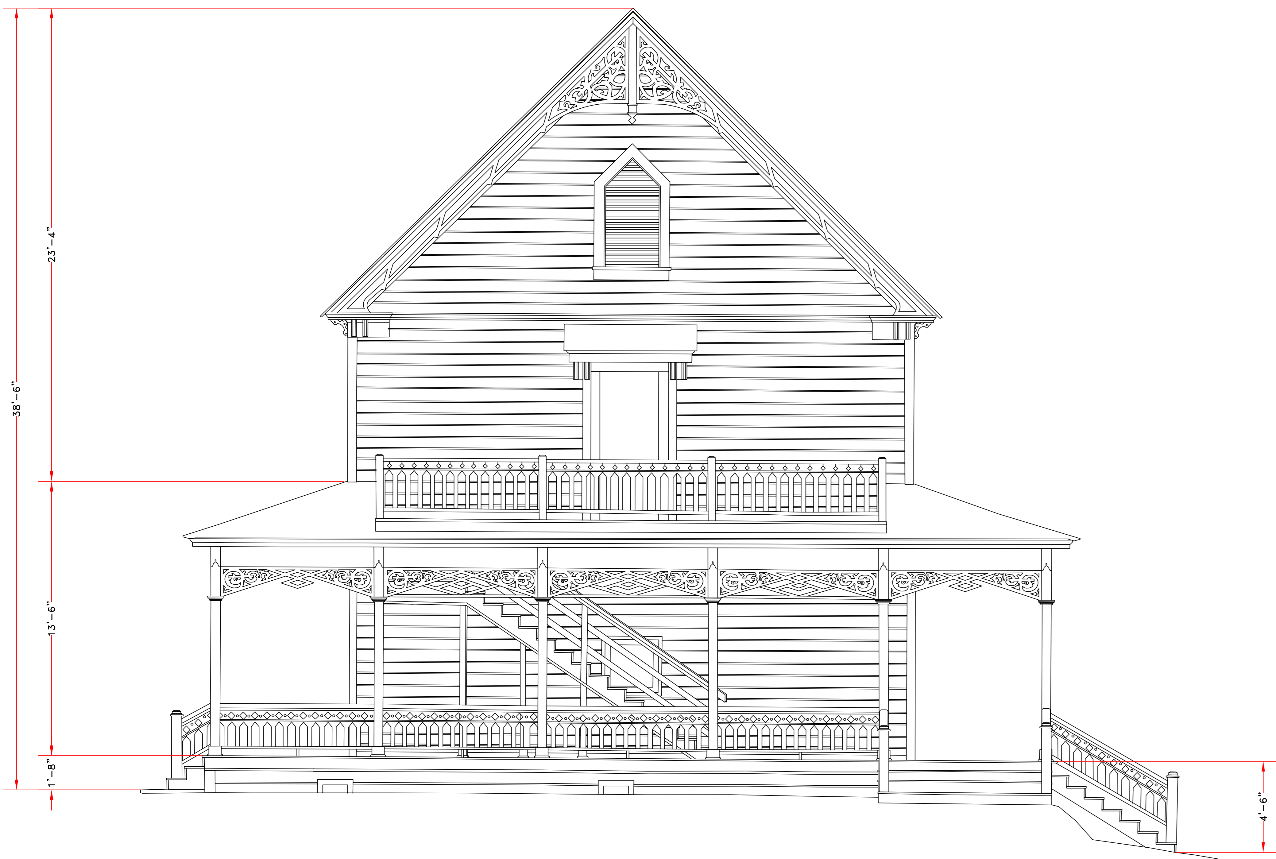
NORTH ELEVATION
